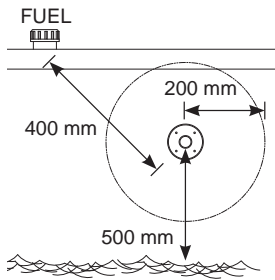
Safety distances
