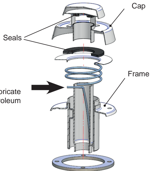
Closable lead-through 2466
