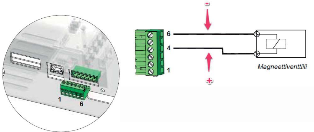
Solenoid valve connection to the circuit board
